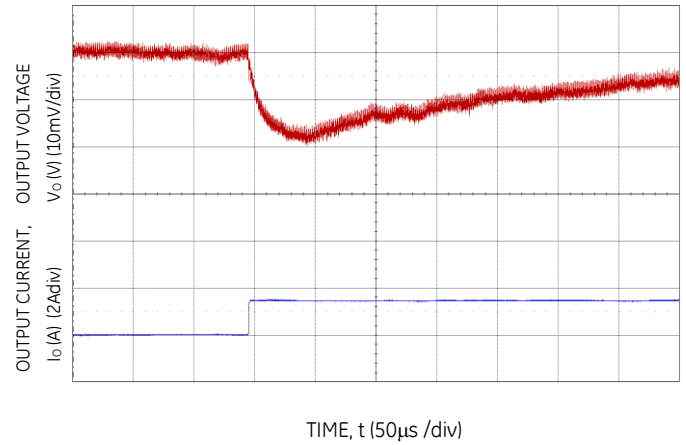
Figure 4. Transient Response to Dynamic Load Change from 50% to 100% at 12V in , C out -2x330μF, 6x100μF, C tune -10nF, R tune -500
