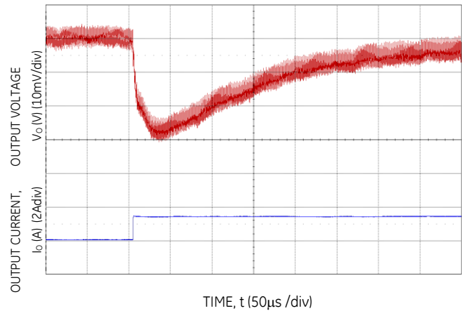
Figure 10. Transient Response to Dynamic Load Change from 50% to 100% at 12Vin, Cout-1x330μF, 4x100μF, Ctune-4.7nF, Rtune-500
