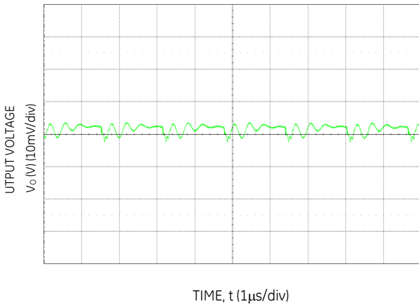
Figure 3. Typical output ripple and noise (C o =88μF ceramic, V IN = 12V, I o = I o,max ).
