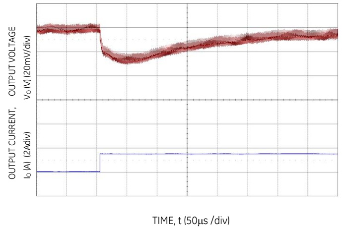
Figure 16. Transient Response to Dynamic Load Change from 50% to 100% at 12Vin, C out -1x330µF, 4x100µF, Ctune-4.7nF, Rtune-500
