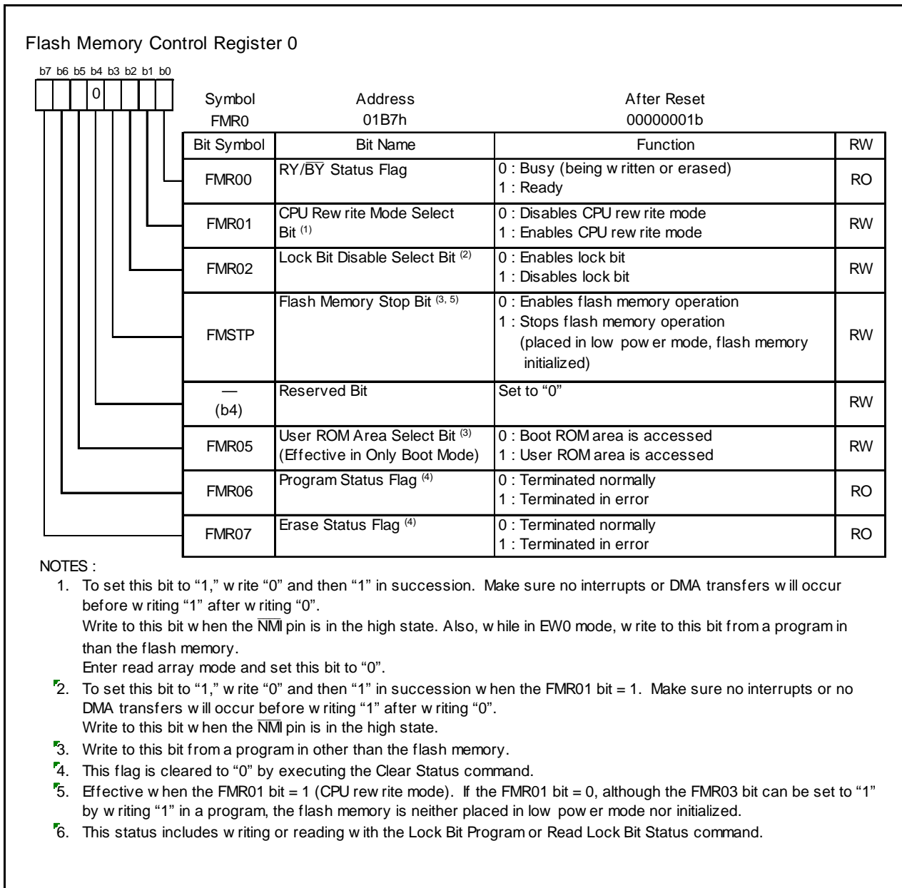
Figure 19.4 FMR0 Register
