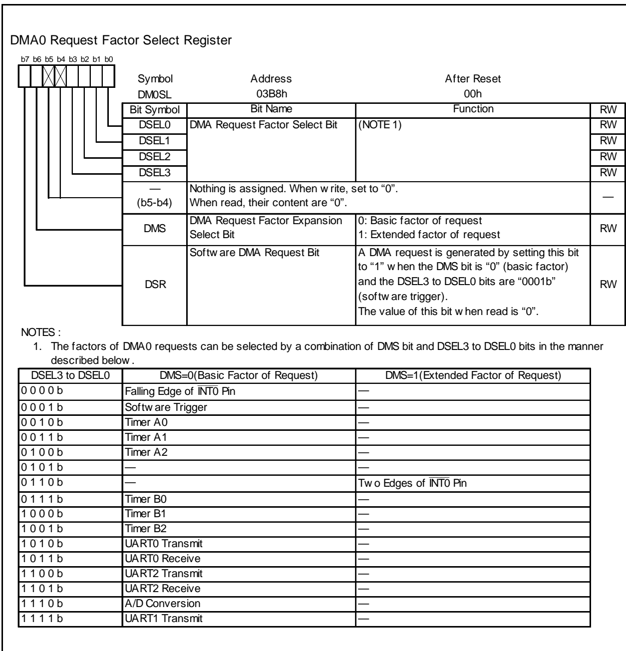
Figure 13.2 DM0SL Register
