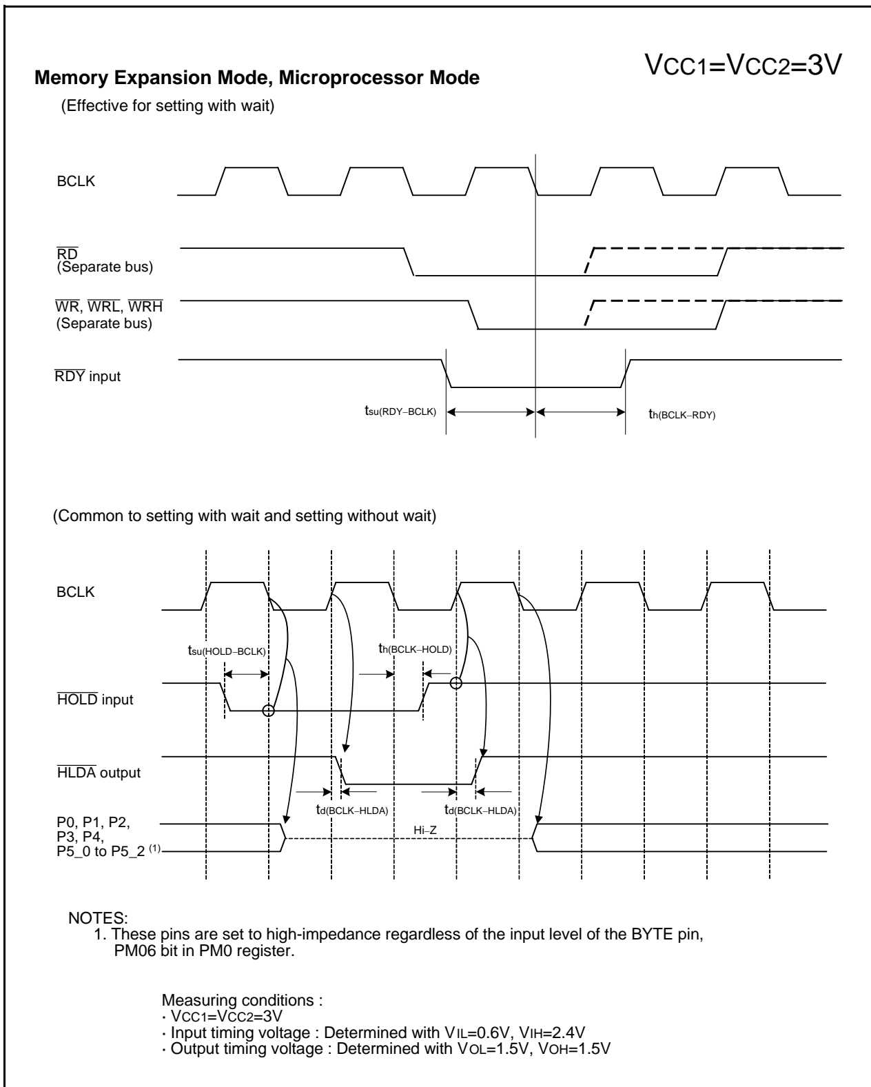
Figure 21.11 Timing Diagram (3)
