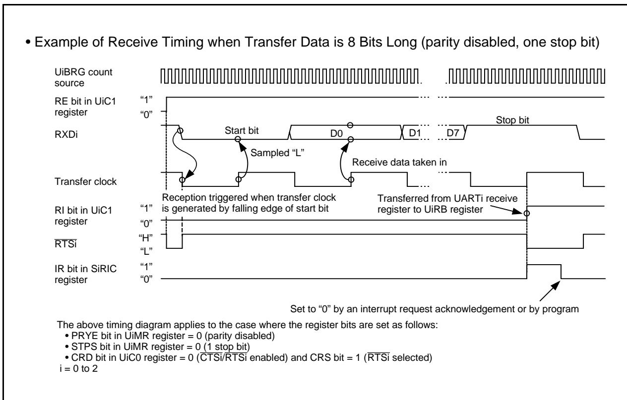
Figure 15.19 Receive Operation
