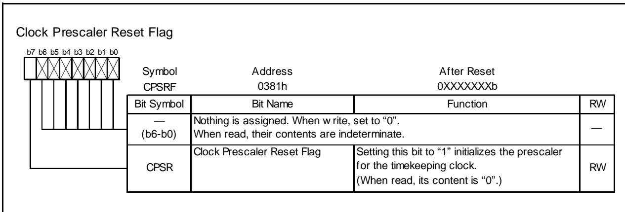
Figure 14.7 CPSRF Register
