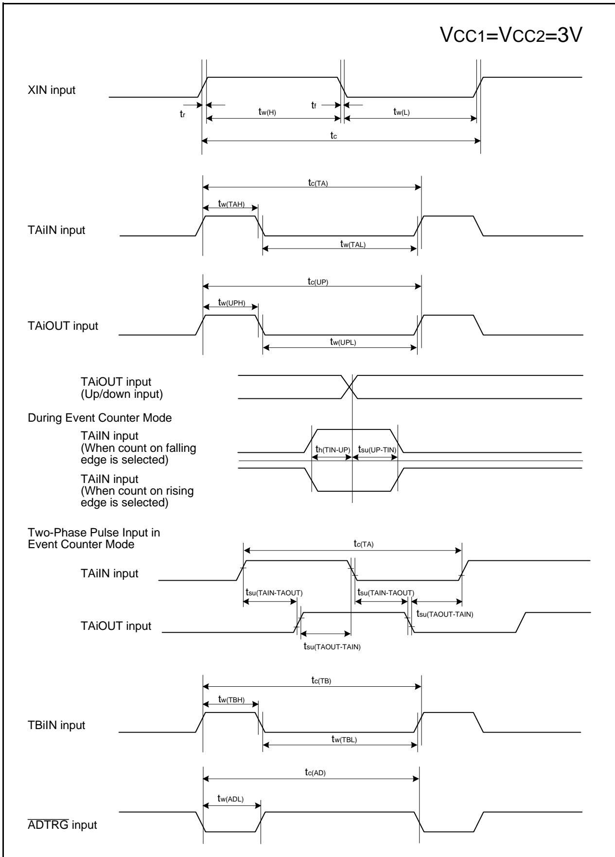
Figure 21.9 Timing Diagram (1)
