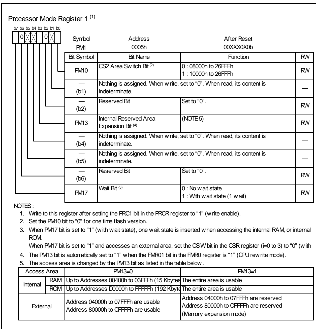
Figure 6.3 PM1 Register (2) (M30304GDPFP, M30304GDPPG, M30304GEPFP, M30304GEPGP, M30302GGPFP, M30302GGPPG)
