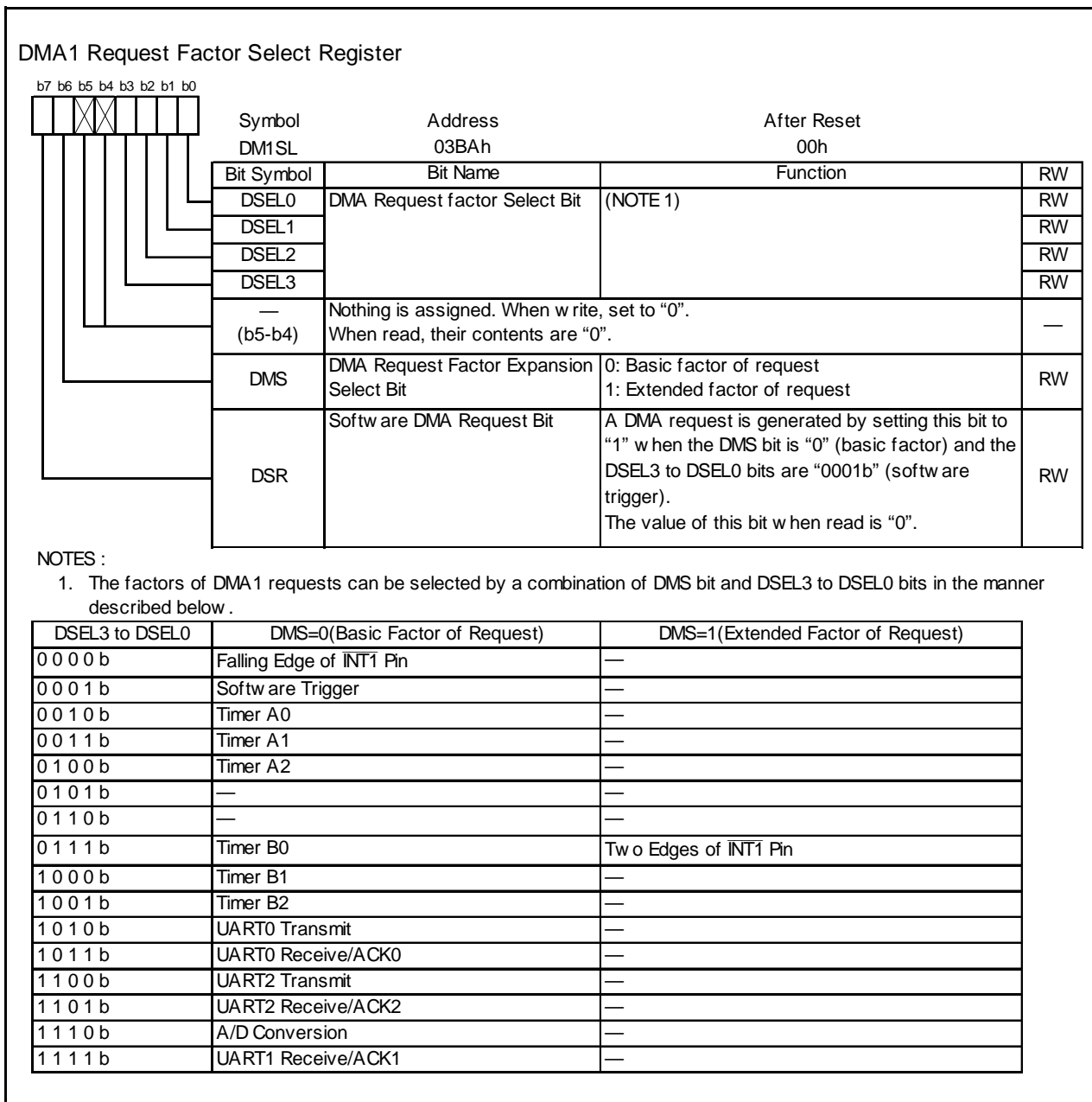
Figure 13.3 DM1SL Register
