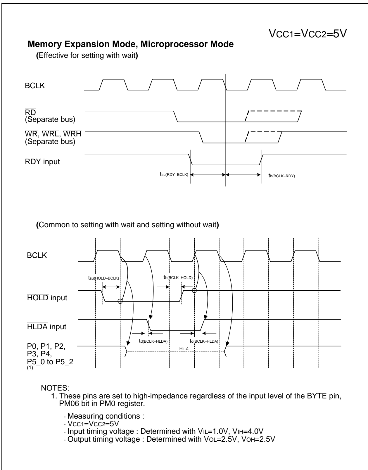
Figure 21.5 Timing Diagram (3)
