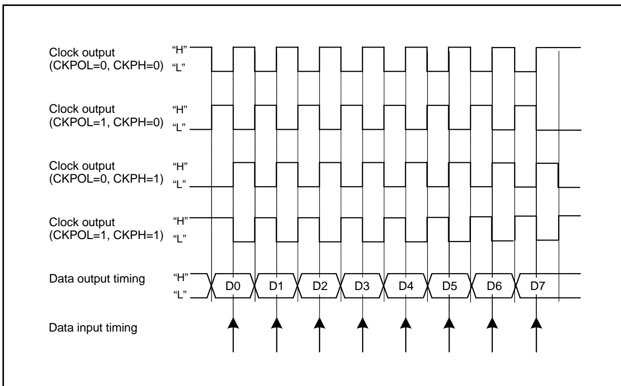
Figure 15.29 Transmission and Reception Timing in Master Mode (Internal Clock)
