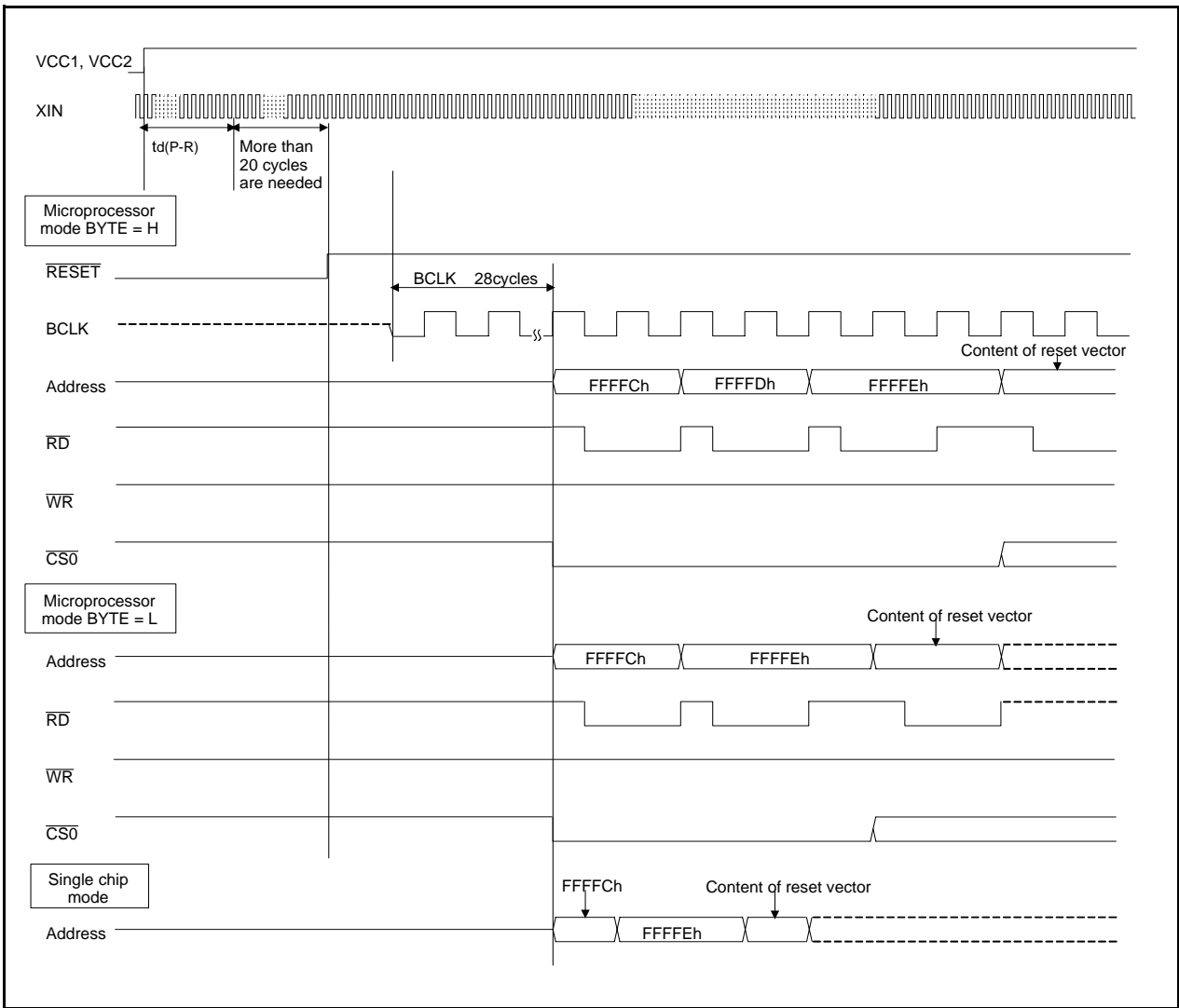
Figure 5.2 Reset Sequence
