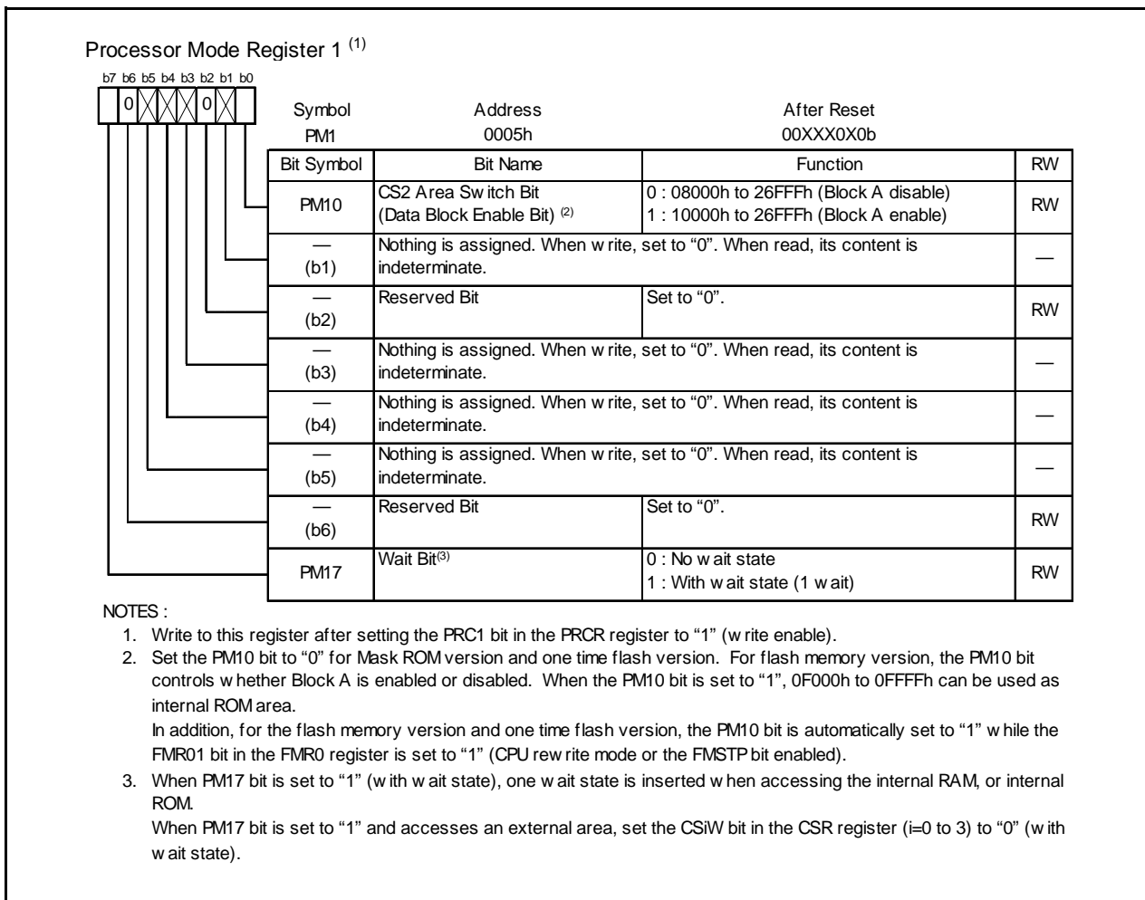
Figure 6.2 PM1 Register (1)
