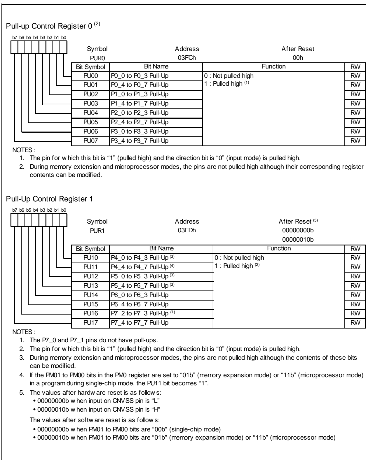
Figure 18.9 PUR0 to PUR1 Registers
