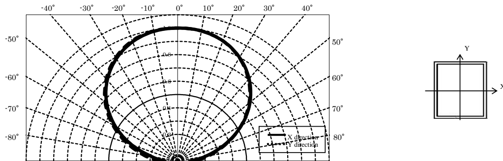
Directive Characteristic
