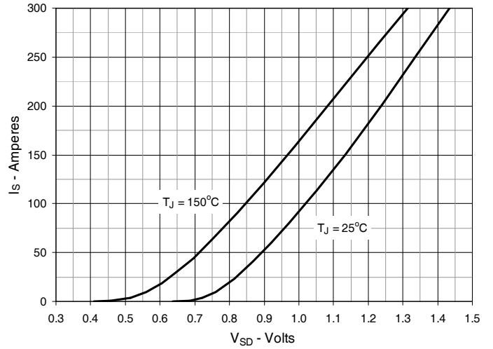
Fig.89. Forward Voltage Drop of Intrinsic Diode
