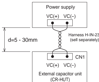
Fig.6.7 Connection method
