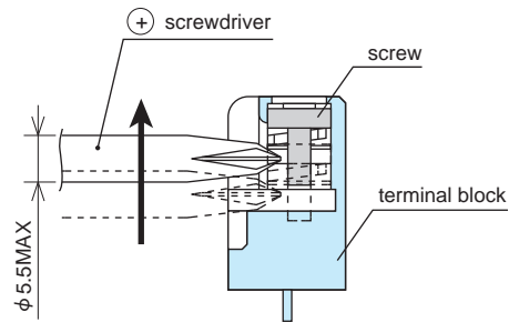
Fig.6.3 lifting method
