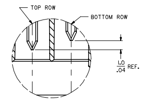
VIEW "Z" SHOWN AFTER TERMINAL INSTALLATION BY CUSTOMER
