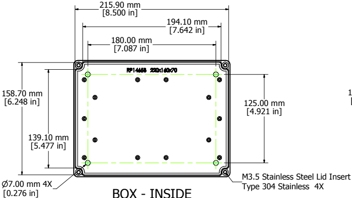
BOX - INSIDE
