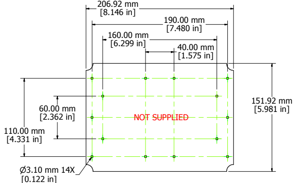
INNER PANEL
