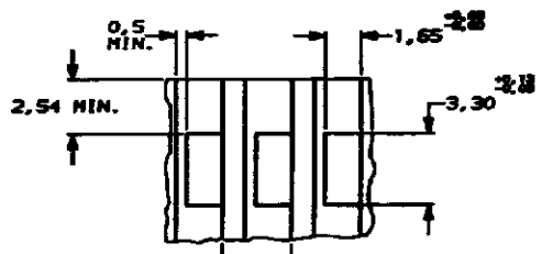
PWB LAYOUT
