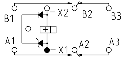
TERMINAL VIEW
