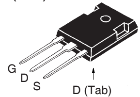
TO-247 (IXFH)
