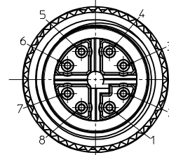
Wiring Scheme M12
