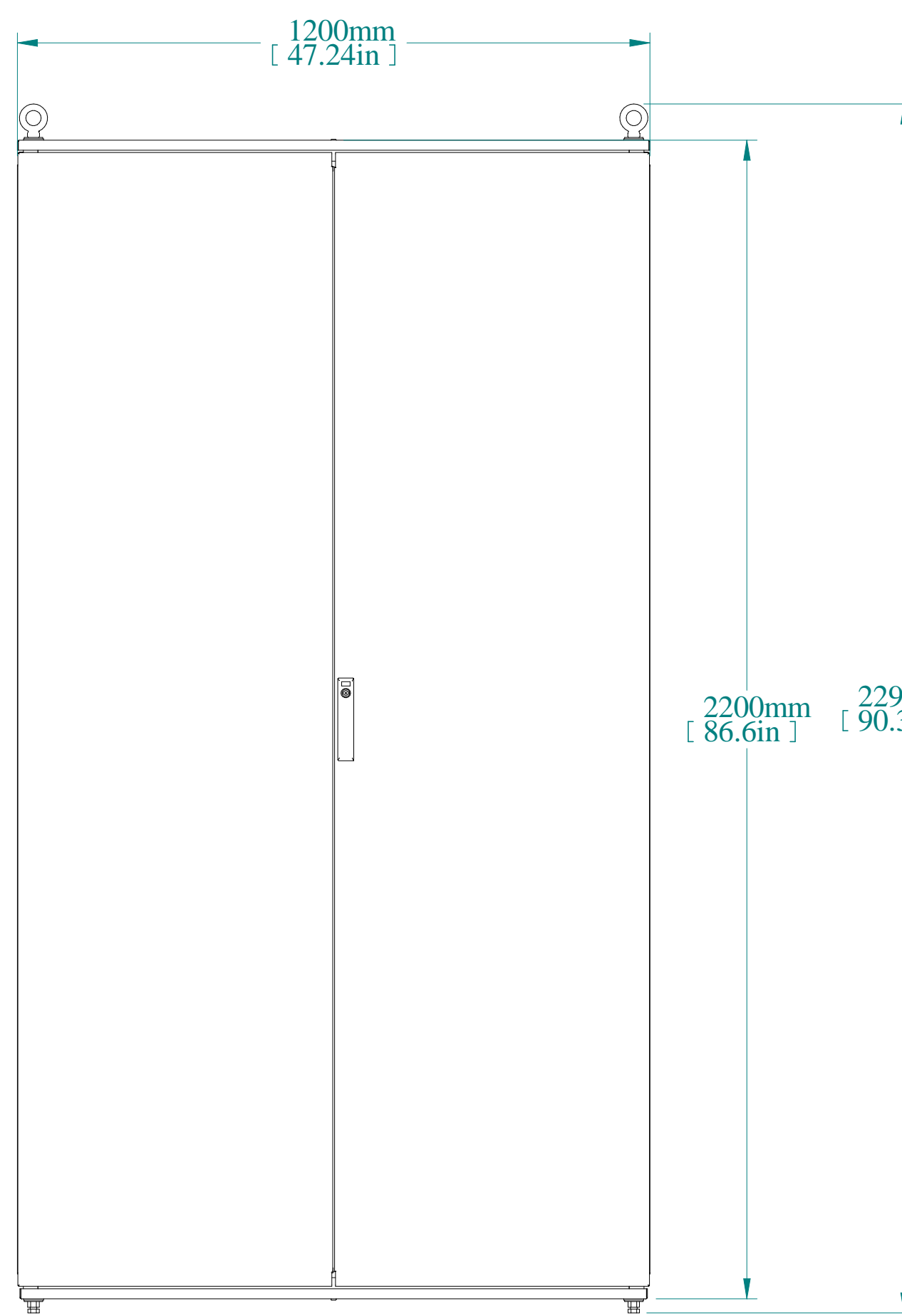
FRONT VIEW
