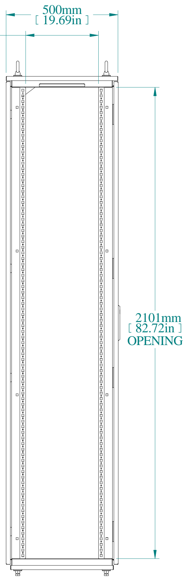
L.S. VIEW
