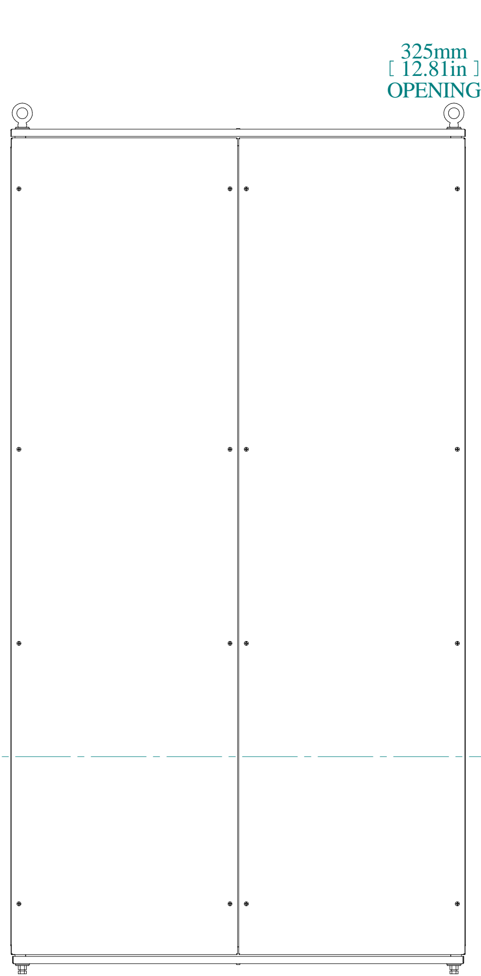
REAR VIEW
