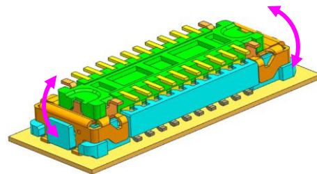
左右に少しずつ振りながら抜く（長手方向） Releasing the plug by moving slowly in "a" direction. (lengthways)
