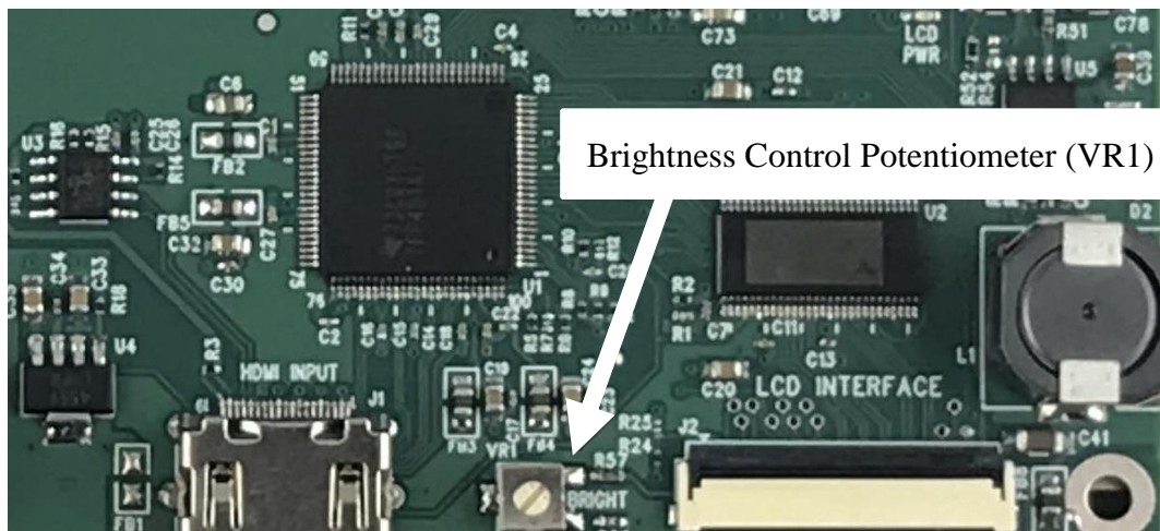
Figure 4. Brightness Control Potentiometer (VR1).
