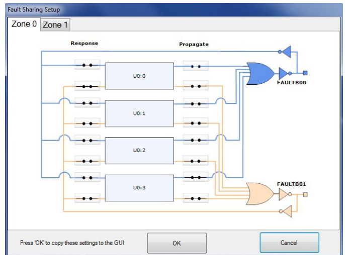
Figure 10. Fault Sharing Utility in LTpowerPlay GUI
