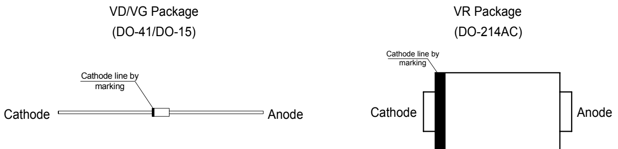
Figure 2. Pin Configuration of APD245
