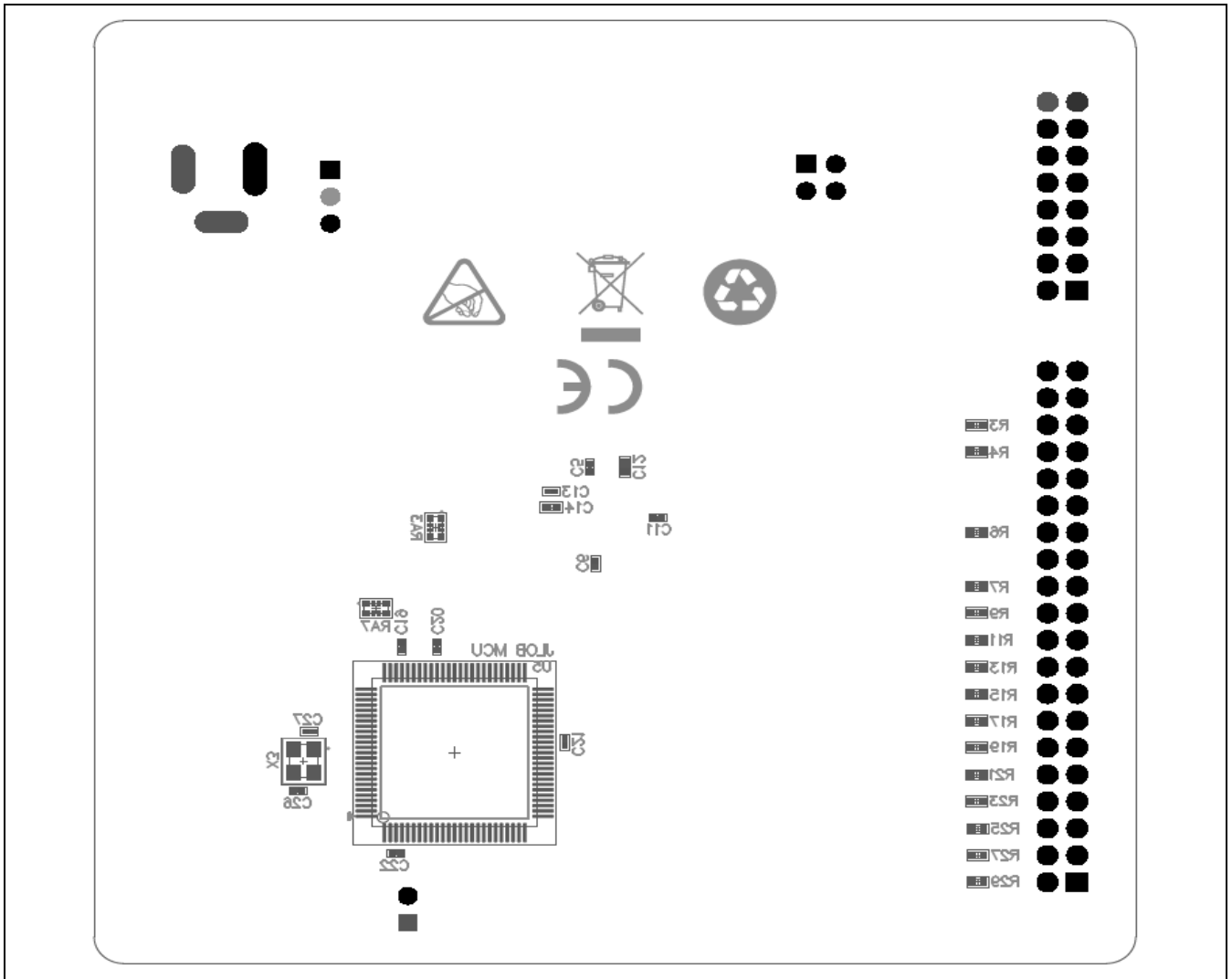
Figure 8 AE-CAP1-S1 Target Board Component Placement, Bottom
