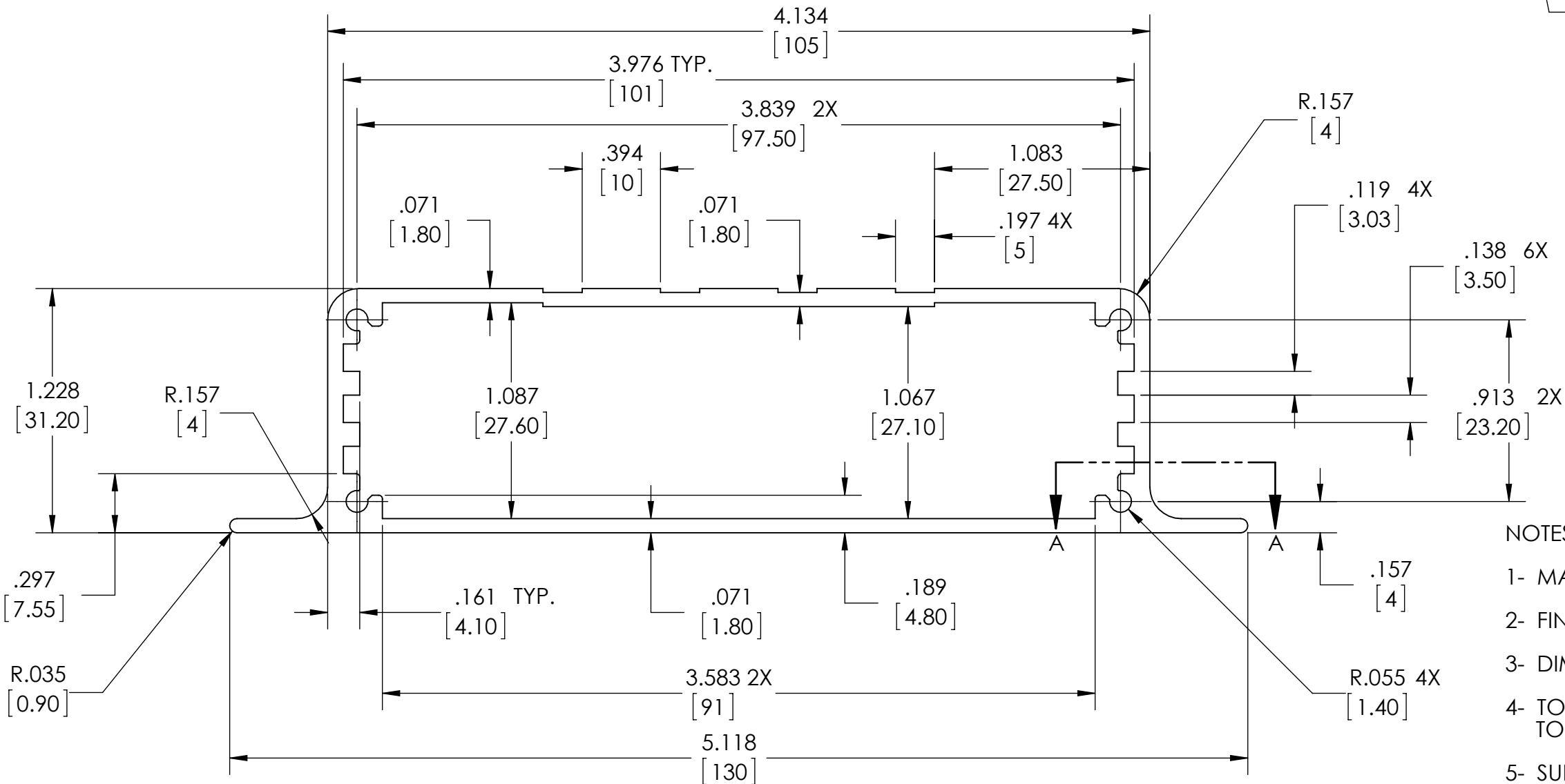
EXTRUSION PROFILE
