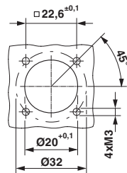
Drill holes
