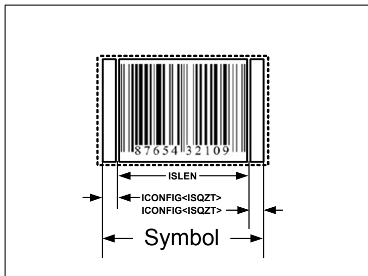
Figure 41: IRBeam Symbol
