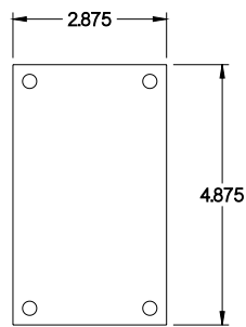
INNER PANEL
