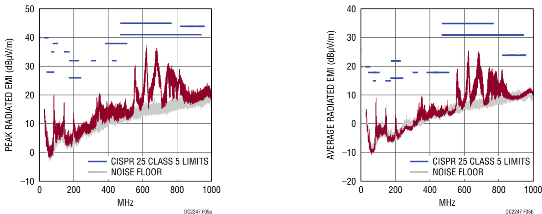
Figure 5. DC2247A Radiated Peak and Average EMI—30MHz to 1GHz—Passes CISPR 25 Class 5 Limits
