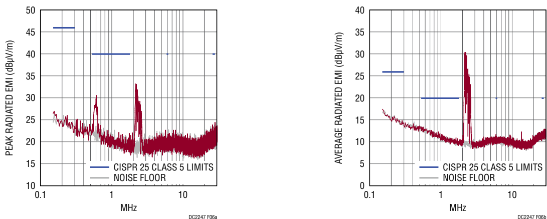
Figure 6. DC2247A Radiated Peak and Average EMI—150kHz to 30MHz—Passes CISPR 25 Class 5 Limits
