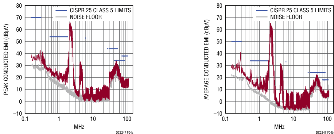
Figure 4. DC2247A Conducted Peak and Average EMI—Passes CISPR 25 Class 5 Limits.
