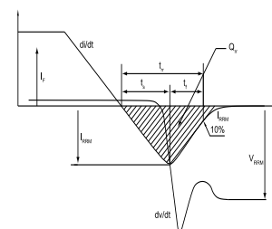
Figure 32: Diode reverse recovery waveform
