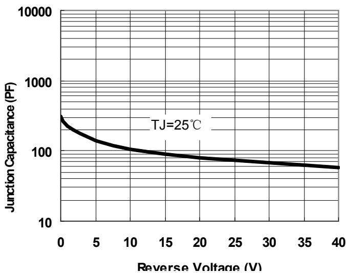
Fig.1-Typical Junction Capacitance
