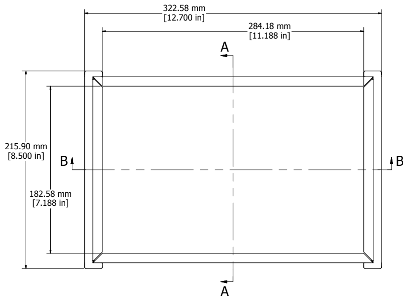
Assembly - View From Bottom
