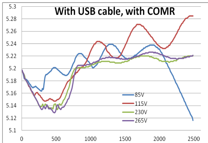
Figure 11. Enable COMR, CV Curve Measure, End of Cable
