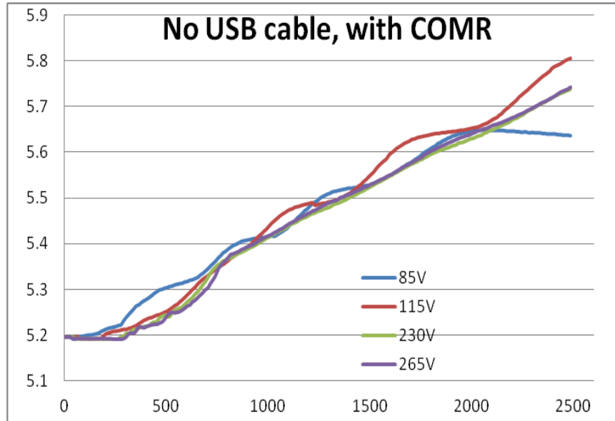
Figure 10. Enable COMR, CV Curve Measure, End of Board
