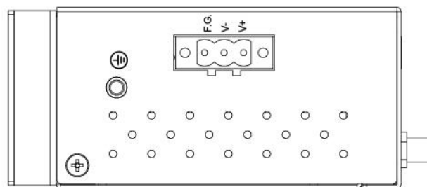
Figure 3.4 Power Panel of all MW550XC Series
