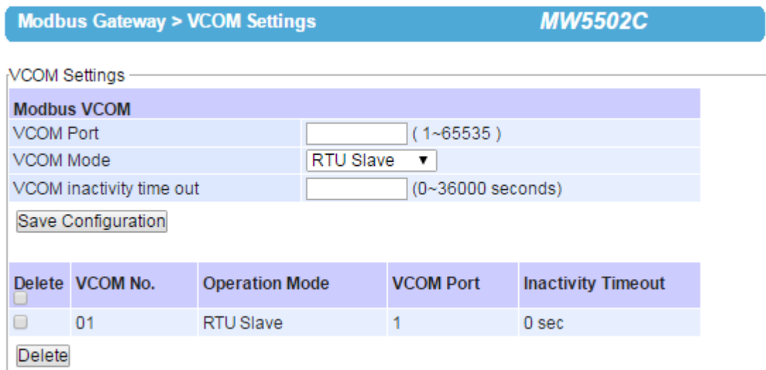
Figure 4.44 VCOM Settings after Save Configuration
