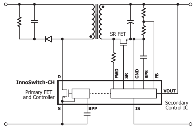
Figure 1. Typical Application/Performance.
