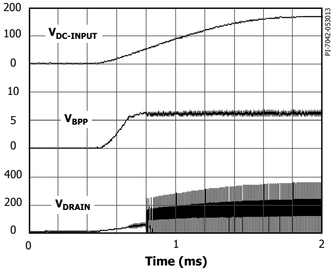
Figure 12. Power-Up Timing.
