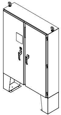
ISOMETRIC VIEW
