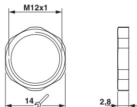
Dimensional drawing
