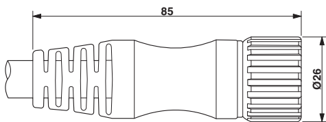
M23 socket, straight, shielded
