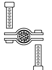
STRAIN RELIEF MOUNTING DETAIL
