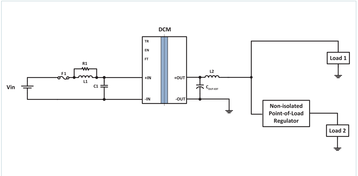
Typical Application: Single DCM3623xA5N53B4y7z, to a non-isolated regulator, and direct to load
