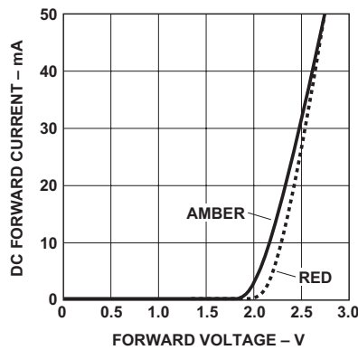
Figure 3b. Forward current vs. forward voltage for option -xxTx red, and option -xxRxx and -xxSxx amber.
