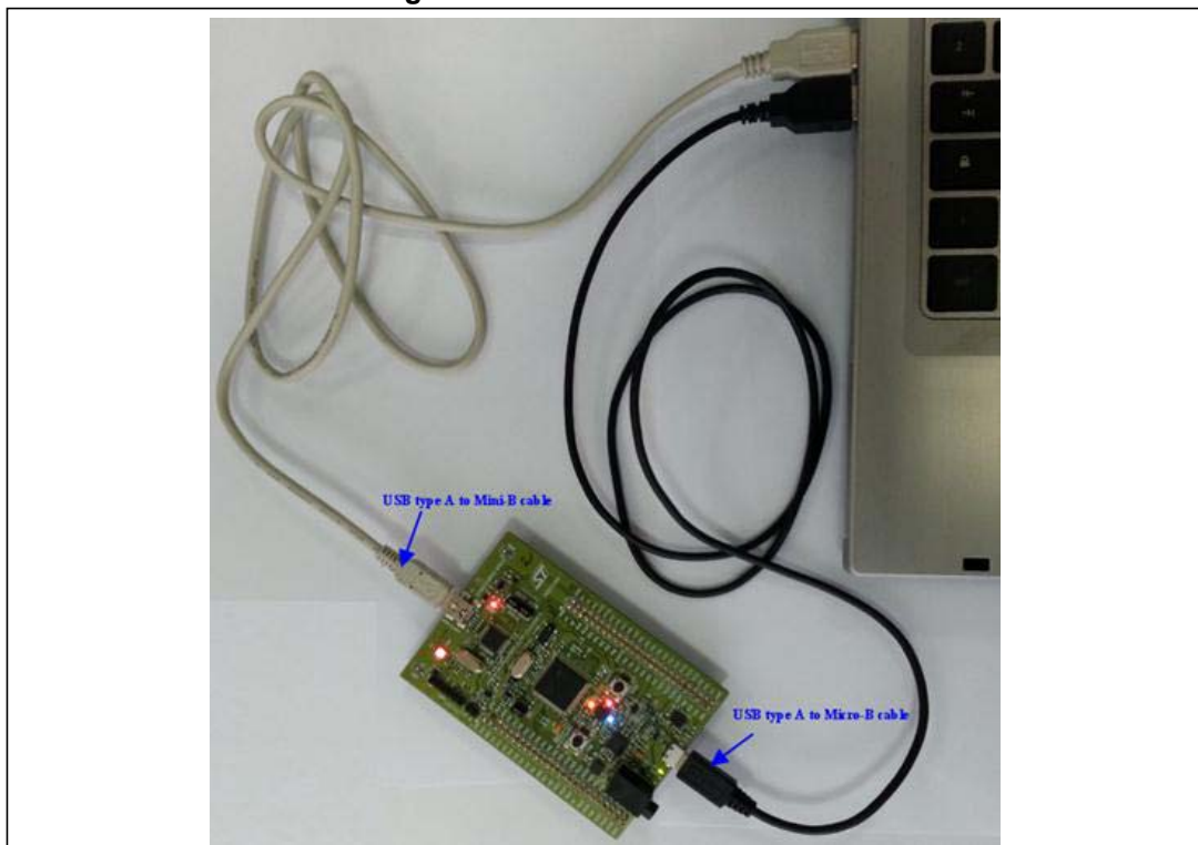
Figure 5. Hardware environment
